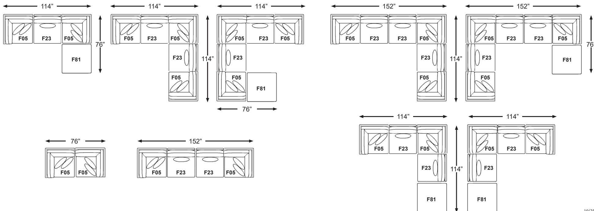
2558-F05 Corner Coin L-38" x D-38" x H-36"
